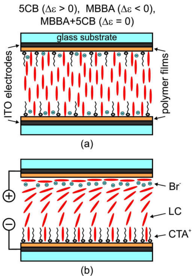
Figure 2. The scheme of the LC orientational transition induced by the electrically controlled ionic modification of surface anchoring. Under the dc electric field, LC is reoriented from the initial homeotropic configuration (a) into the hybrid one (b) independently on the sign and value of the dielectric anisotropy \Delta\varepsilon of the used nematic.
