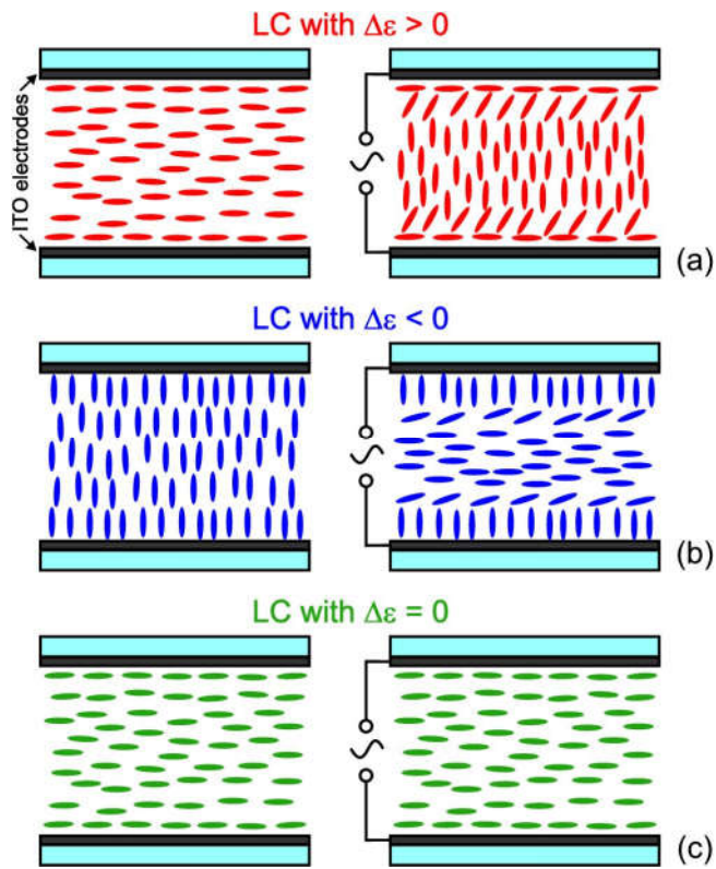
Figure 1. The Frederiks effect in LC cells based on the nematics with positive (a), negative (b) and zero (c) dielectric anisotropy induced by the electric field. The initial LC orientations are shown in the left column. The right column represents LC orientations under the action of the ac electric field applied perpendicularly to the substrates.
