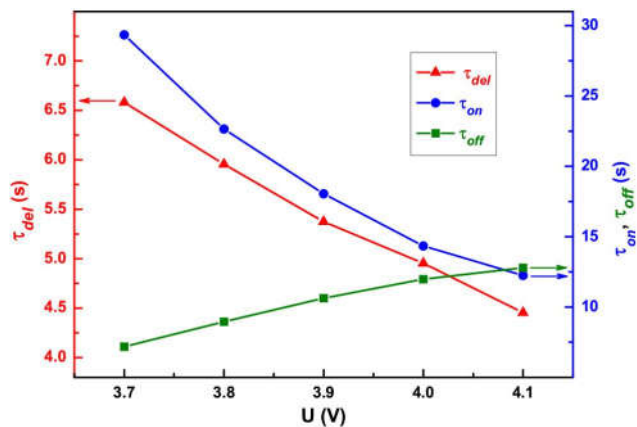
Figure 4. Delay time \tau_{del} (left axis), turn-on time \tau_{on} and turn-off time \tau_{off} (right axis) depending on the control voltage for the LC cell based on the MBBA-5CB mixture ( \Delta\varepsilon = 0 ) doped with CTAB.
