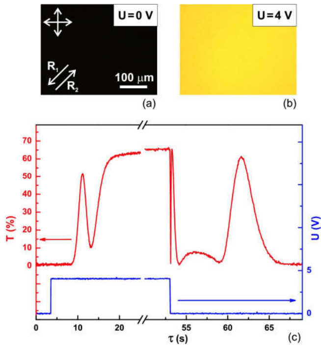
Figure 3. Optical textures of the LC cell based on the MBBA-5CB mixture ( \Delta\varepsilon = 0 ) doped with CTAB in the initial state (a) and under the dc electric field 4 V (b); the square-wave optical response of the LC cell (the top curve) placed between the crossed polarizers and electric 4 V pulse (the bottom curve) (c). The polarizer directions are shown by the double arrows. \mathbf{R}_1 and \mathbf{R}_2 are rubbing directions of the top and bottom substrates, respectively.
