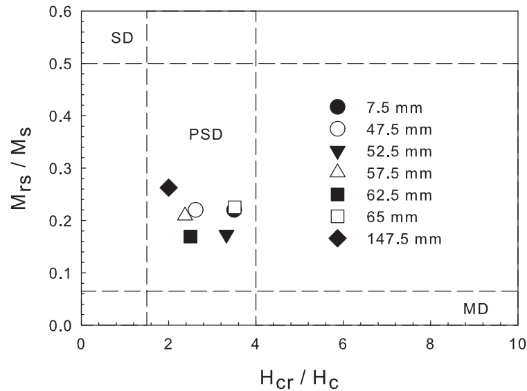
Figure 3: The Day plots for the studied samples from the sediments of various depths.
