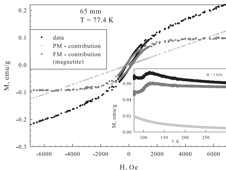
Figure 1: Typical results of magnetic measurements of a sediment at the depth of 65 mm together with FM and PM contributions.
