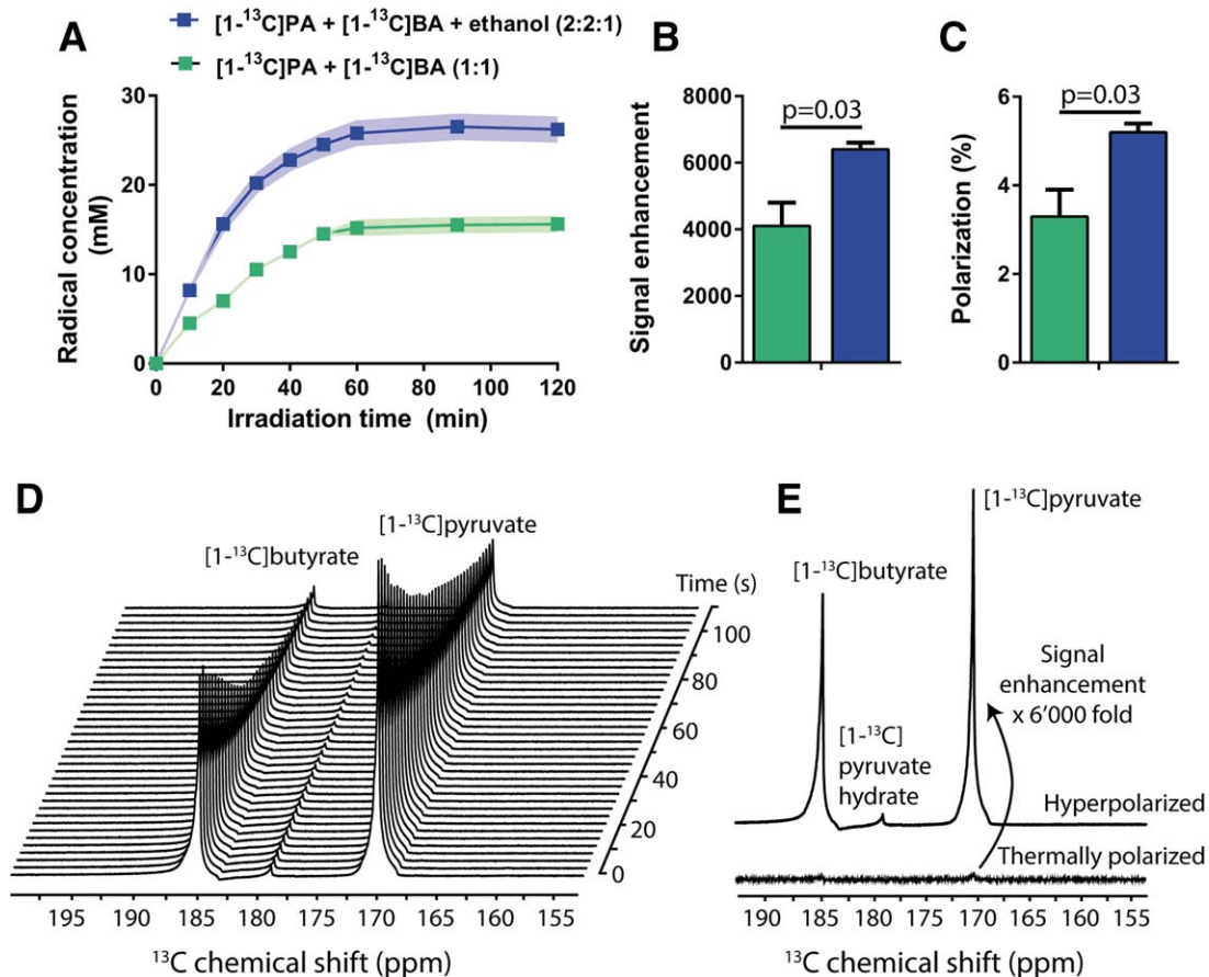
FIGURE 2 A, Radical concentration as a function of the UV light irradiation time for 2 different mixtures: [1- ^{13}\text{C} ]pyruvic- and [1- ^{13}\text{C} ]butyric acids in a 1:1 volume ratio (green), and the same with the addition of ethanol (blue). Signal intensity enhancement (B) and polarization levels (C) of pyruvic acid using 2 differently prepared mixtures. D, E, In vitro hyperpolarized ^{13}\text{C} MRS of the UV-irradiated mixture of ^{13}\text{C} labeled substrates. D, Hyperpolarized ^{13}\text{C} spectral time course of the mixture measured in the infusion pump inside the MRI scanner after dissolution and automated sample transfer. Hyperpolarized spectra were acquired with an RF excitation angle of 5^\circ and TR of 3 seconds. E, The first measured hyperpolarized ^{13}\text{C} spectrum after dissolution (top spectrum) was compared with its thermally polarized counterpart (bottom spectrum) to calculate the SNR enhancement in liquid state. A 6'000-fold signal enhancement was measured. All spectra are displayed without spectral line broadening
