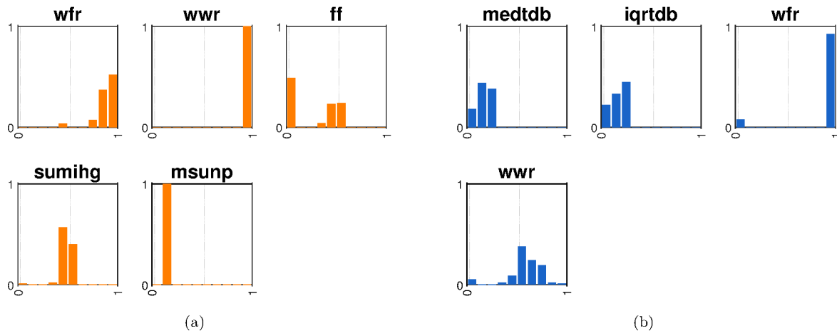
Figure 3: Empirical estimates of the relevance parameters 1/l_i for significant input variables heating (Figure 3a) and cooling (Figure 3b) loads. A value of 1/l_i close to zero, for a particular input, indicates that that input was not involved in determining the prediction of the model. A significant input is one for which at least one non-zero value of 1/l_i has a relative share greater than 20% of the total samples. The title of each plot is the variable code (see Table 2 for an explanation of the variable codes). The histogram is obtained from the 100 runs over training-data subsets of size N_{train} = 4,000 .
