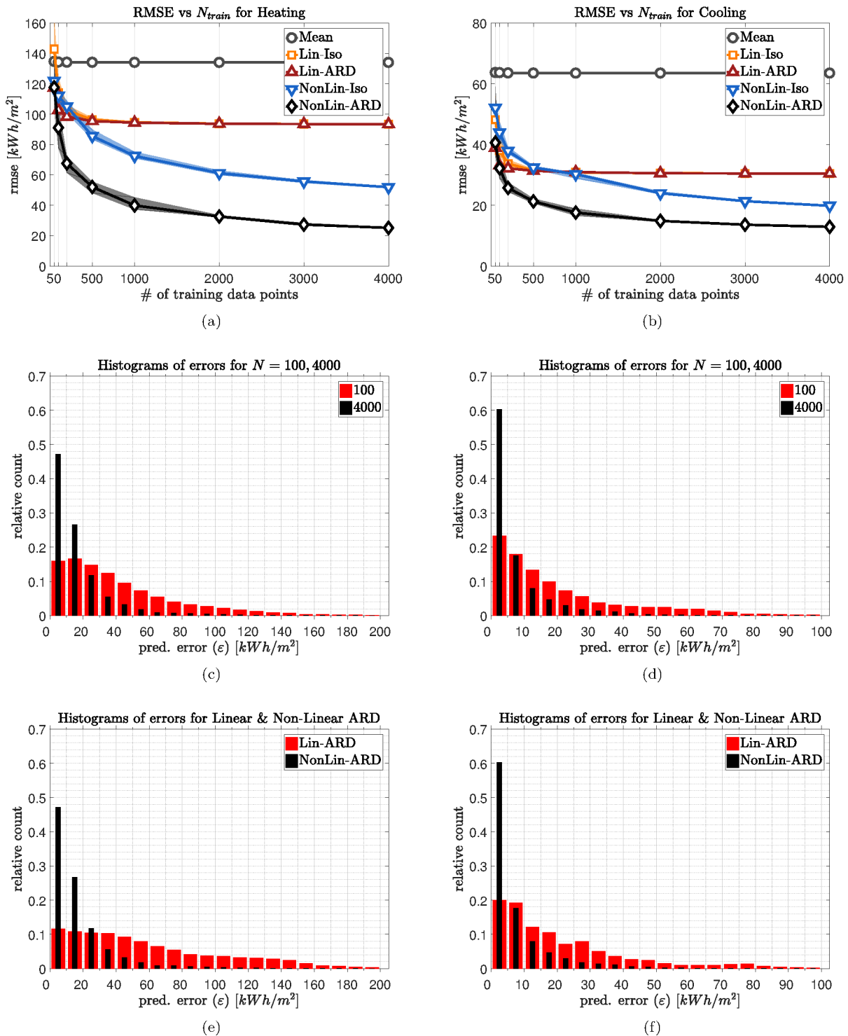
Figure 2: Plots on the left show results for the heating loads and on the right show results for the cooling loads. Figures a and b show the Root Mean Square Error (RMSE), plotted against the size of the training data set. The lines indicate median errors, and the filled areas are bounded by the 25th and 75th percentiles. The non-linear models outperform linear models, and the predictions improve with size of training data set. Figures c and d compare the empirical estimates of distributions of absolute errors, |\epsilon| = |y_j - f_e(\mathbf{x}_j)| , for N_{train} = 100 and 4,000. We see that a large training data size reduces larger values of error. Figures e and f compare the same for the linear and non-linear models, where we see that the nonlinear model makes fewer errors.
