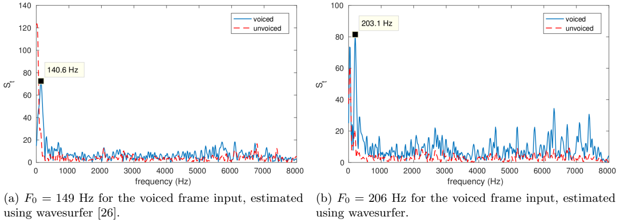
Figure 4: Filters response for voiced and unvoiced male speech and female speech frame inputs.
