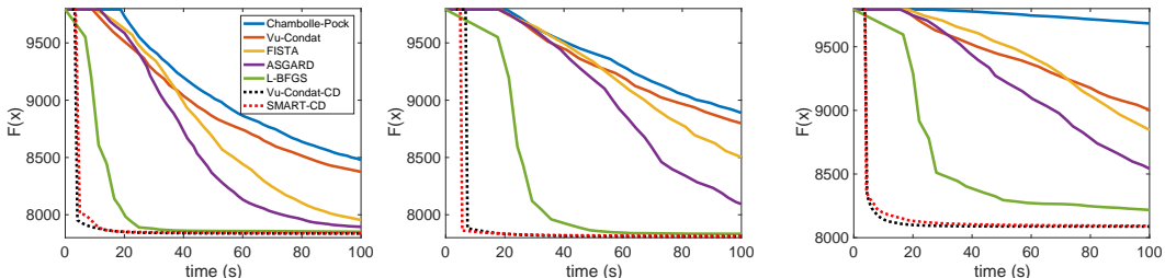
Figure 2: The convergence of 7 algorithms for problem (18). The regularization parameters for the first plot are \lambda = 0.001, r = 0.5 , for the second plot are \lambda = 0.001, r = 0.9 , for the third plot are \lambda = 0.01, r = 0.5 .
