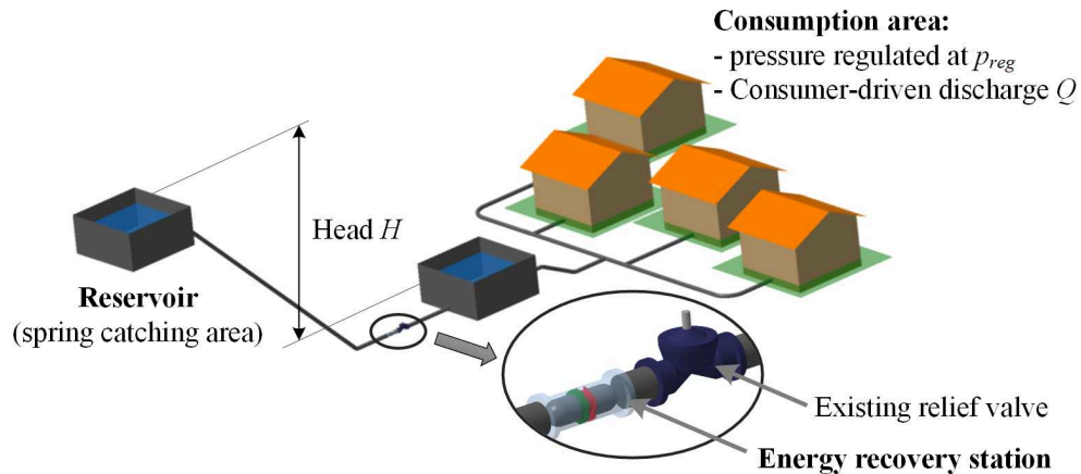
Figure 1. Water utility network with hydro power potential.
