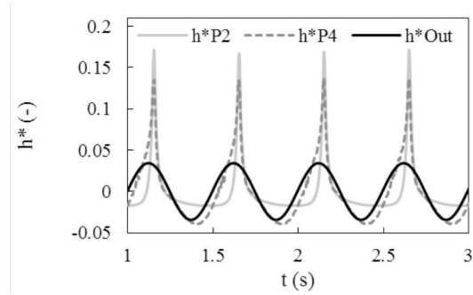
Figure 7. Venturi: Pressure fluctuations in resonance conditions obtained by CFD ( f_s = 2\text{Hz} ).
