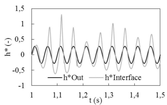
Figure 9. Francis turbine: Pressure fluctuations in resonance conditions obtained by CFD ( f_s = 20\text{ Hz} ).
