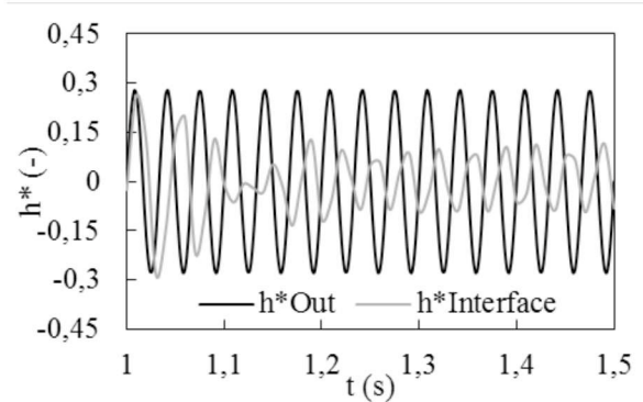
Figure 8. Francis turbine: Pressure fluctuations in out of resonance conditions obtained by CFD ( f_s = 30\text{ Hz} ).
