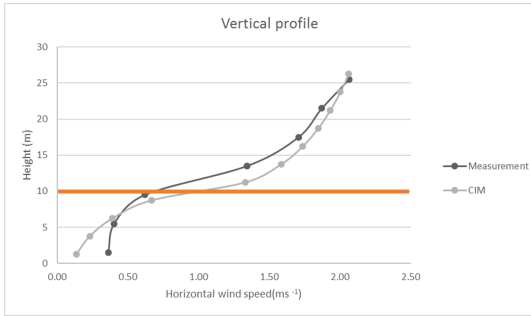
Fig. 3 – Vertical profile of the horizontal wind speed ( ms^{-1} ) from the sonic anemometers (in black) and results from CIM (in grey) with the height (m) on the vertical axis. Orange line represent the building height (10 m).
