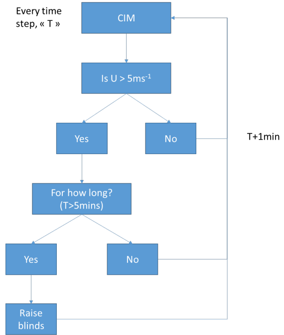
Fig. 2 – Proposed algorithm flow chart.
