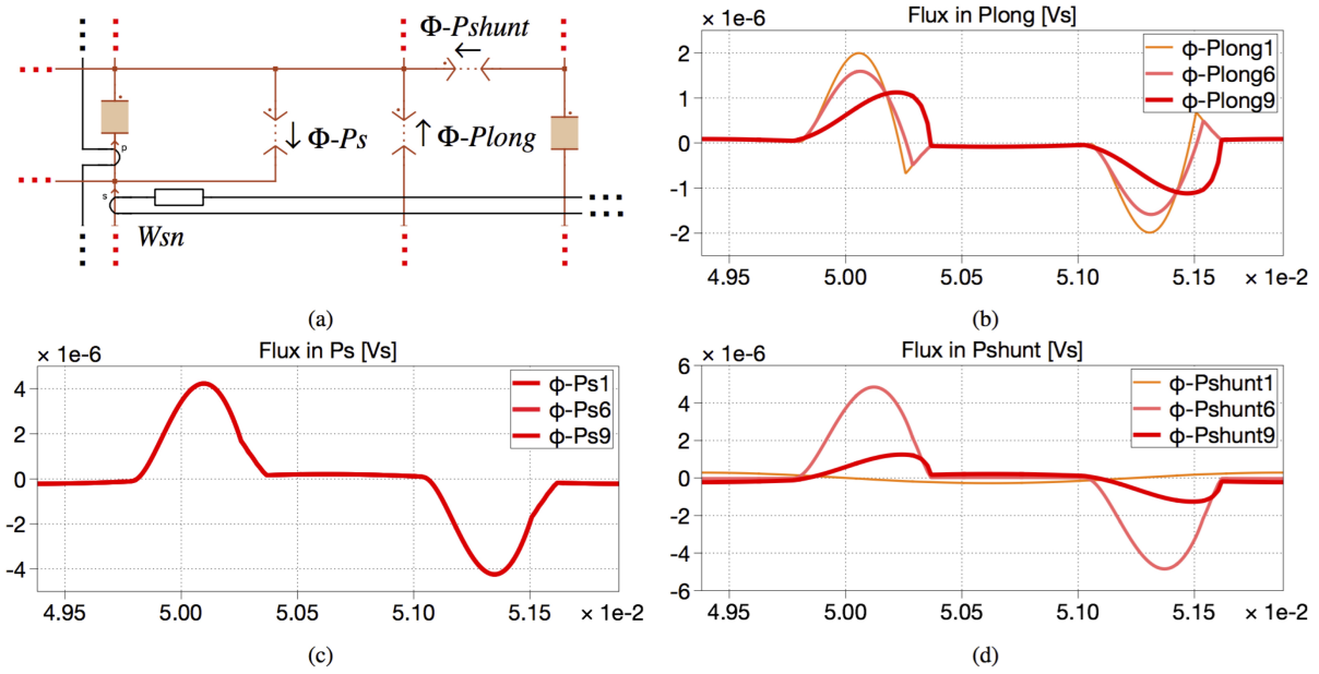
Fig. 23: Simulated flux in the magnetic circuit divisions including secondary windings W_{s1} , W_{s6} and W_{s9} (a) Illustration of flux measurement positions in each magnetic circuit division (b) Simulated flux on P_{long} (c) Simulated flux on P_s (d) Simulated flux on P_{shunt}
