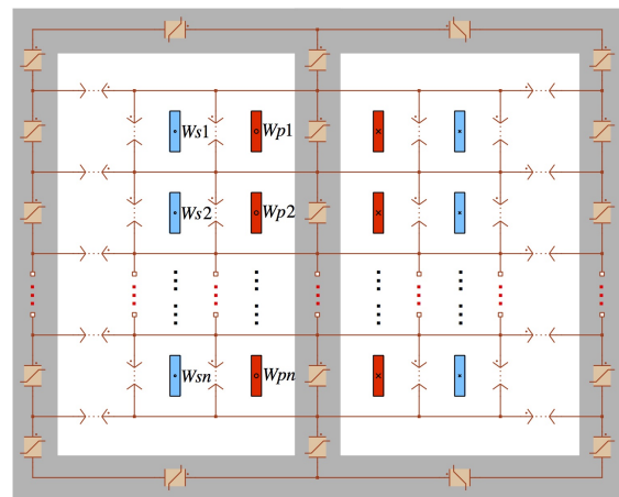
Fig. 8: Permeance circuit of the transformer with the horizontal leakage permeances above- or below the windings neglected
