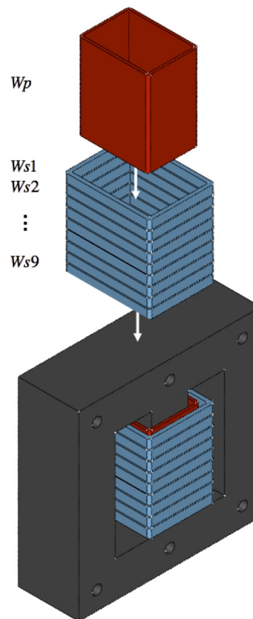
Fig. 3: Structure of the prototype transformer with one primary- W_p and nine secondary windings W_{sk}
