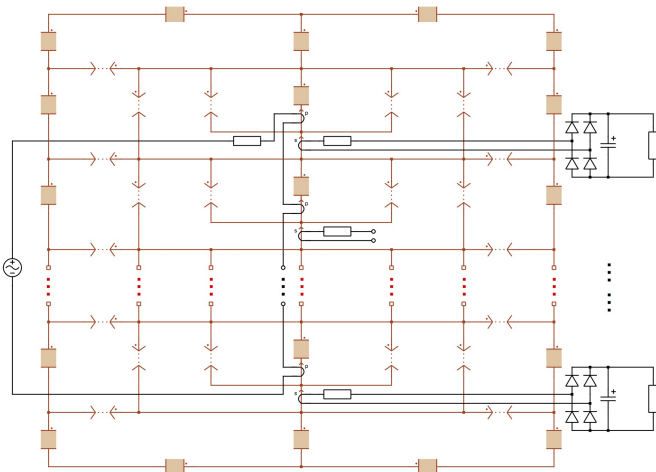
Fig. 20: System-level simulation model with diode rectifiers connected
