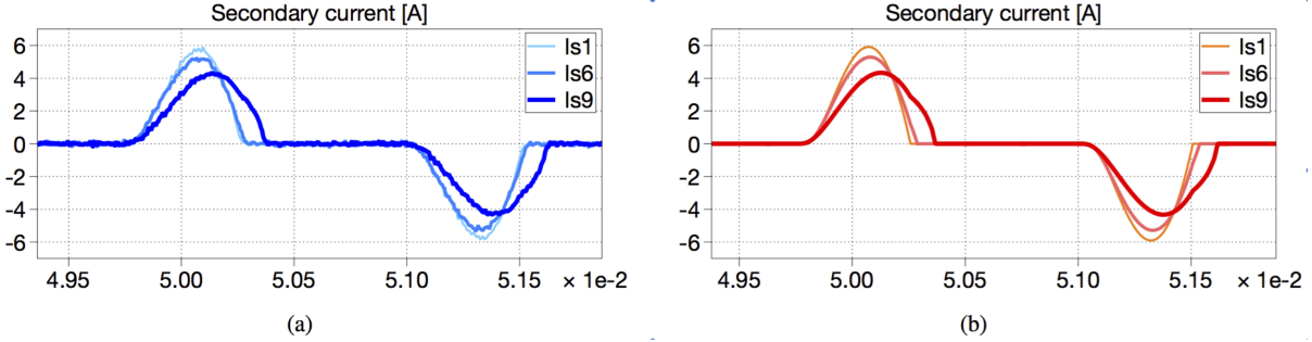
Fig. 22: Secondary winding currents in verification scheme A, with primary winding supplied, secondary windings W_{s1} , W_{s6} till W_{s9} connected to rectifiers, (a) Test measurement (b) PLECS/Simulink simulation
