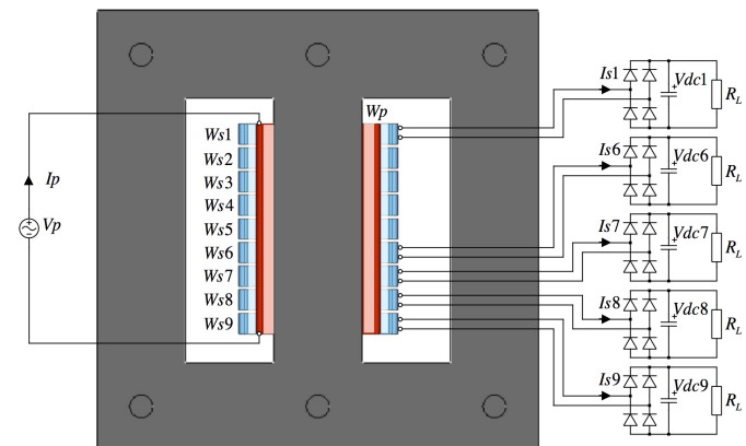
Fig. 18: Schematic of the system-level verification setup with five diode rectifiers connected (configured for verification scheme A with secondary windings W_{s1} , W_{s6} till W_{s9} connected to rectifiers)
