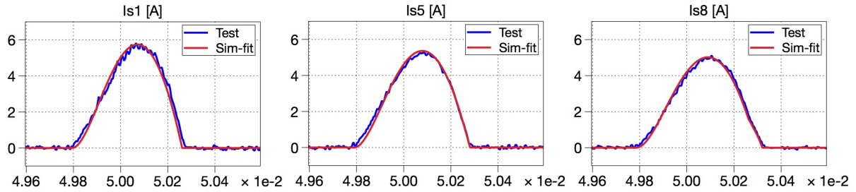
Fig. 24: Comparison of secondary currents in verification scheme B between measurement and simulation
