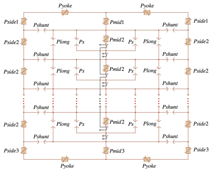
Fig. 10: Final version of the magnetic circuit model
