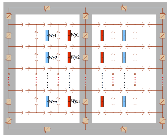
Fig. 7: Original permeance circuit of the transformer with schematically placed windings
