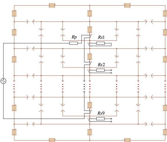
Fig. 14: Magnetic circuit model in PLECS for parameter fitting and verification
