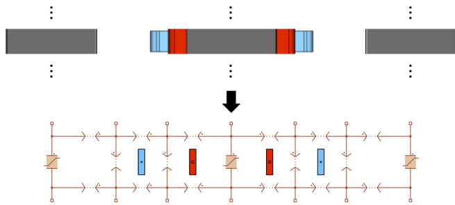
Fig. 5: Permeance magnetic circuit of the division type I with the flux path of the core and air
