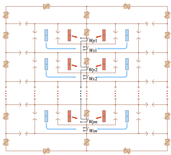
Fig. 9: Permeance circuit with lumped-winding components to interface electrical circuit
