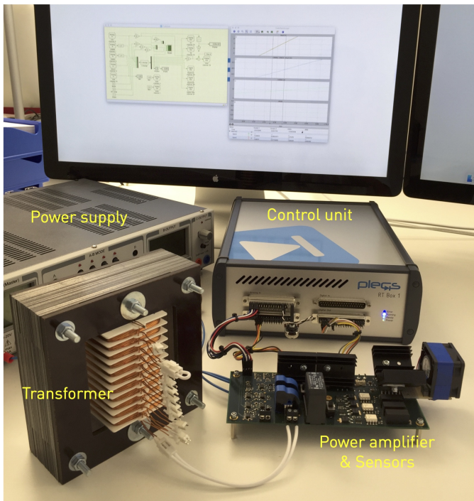
Fig. 13: Short-circuit test setup for the prototype transformer, with voltage and current on the supplied winding measured
