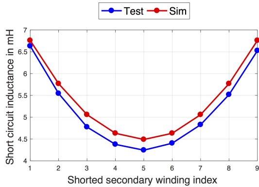
Fig. 15: Short circuit inductances with W_p supplied and different single W_s shorted
