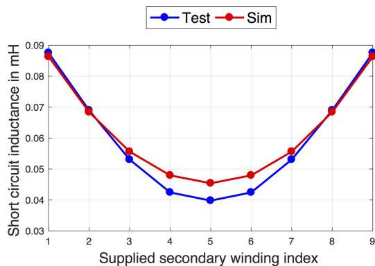
Fig. 17: Short circuit inductances with W_p shorted and different single W_s supplied
