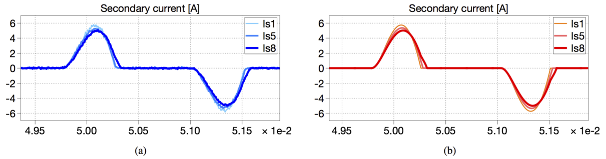
Fig. 25: Secondary winding currents in verification scheme B, with primary winding supplied, secondary windings W_{s1} , W_{s5} till W_{s8} connected to rectifiers, (a) Test measurement (b) PLECS/Simulink simulation
