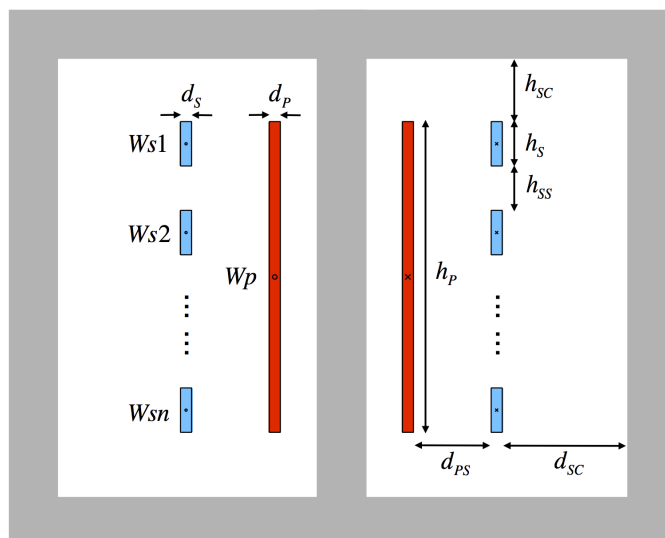
Fig. 2: Winding arrangement with long primary winding and multiple stacked secondary windings
