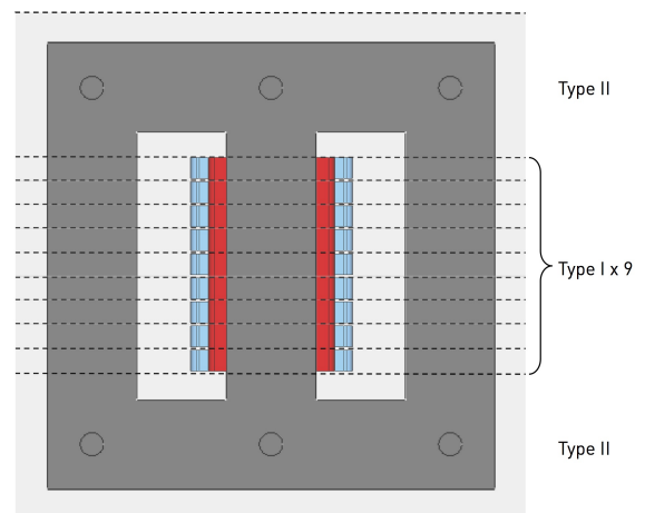
Fig. 4: Vertical separation of the transformer's geometry into nine divisions of type I and two of type II
