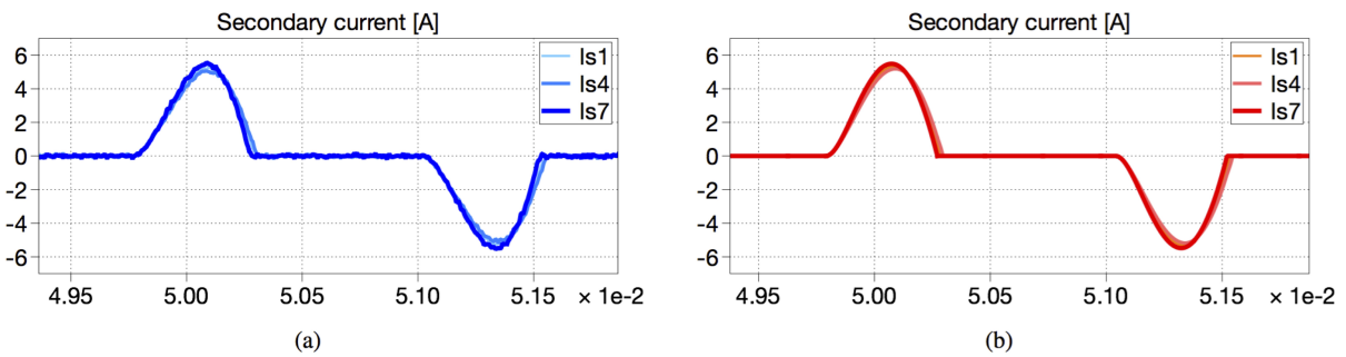
Fig. 27: Secondary winding currents in verification scheme C, with primary winding supplied, secondary windings W_{s1} , W_{s4} till W_{s7} connected to rectifiers, (a) Test measurement (b) PLECS/Simulink simulation
