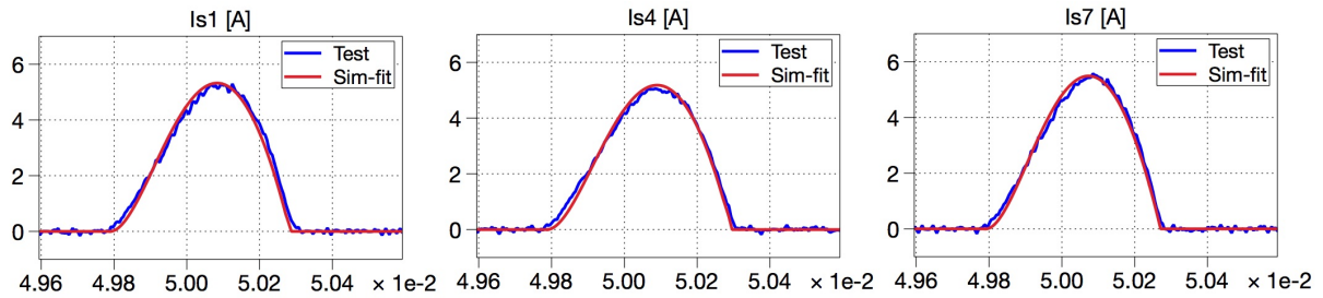
Fig. 26: Comparison of secondary currents in verification scheme C between measurement and simulation
