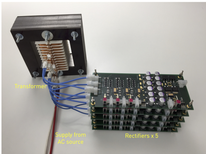
Fig. 19: Photo of the system-level verification setup
