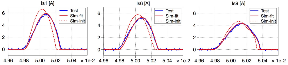
Fig. 21: Comparison of secondary currents in verification scheme A between measurement and simulation (solid curve), additionally to simulation result obtained with initial permeance values (dashed curve)
