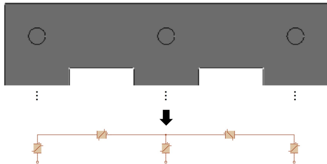
Fig. 6: Permeance magnetic circuit of the division type II
