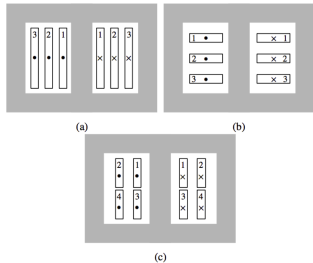
Fig. 1: Winding arrangements considered in the existing publications [9] [10] [11][13], (a) Multilayer (b) Multidisk (c) Mixed
