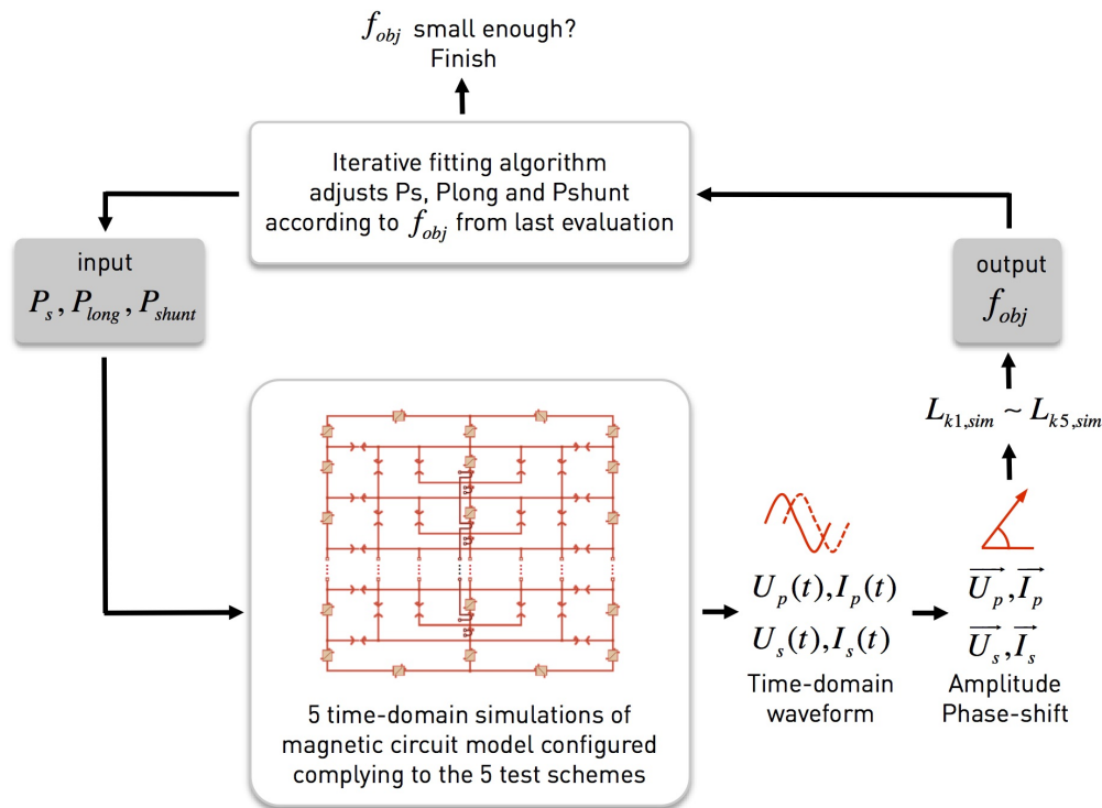
Fig. 12: Generalised fitting process of the leakage permeance values, where the magnetic circuit model is simulated to for calculating the output of the objective function for the fitting algorithm
