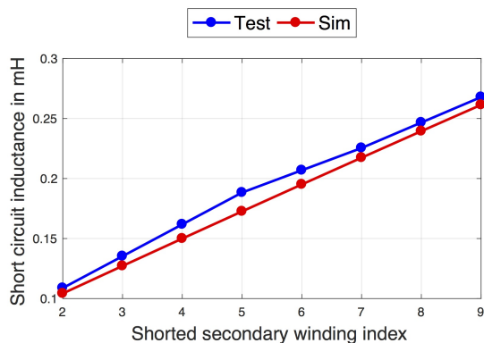
Fig. 16: Short circuit inductances with W_{s1} supplied and one of the other W_{s} shorted
