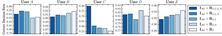
Fig. 9. Performance of five example users obtained on combination of all Image Semantic Features ( \mathbf{I}_{All} ) and different Requester Contextual Features ( \mathbf{R} ).
