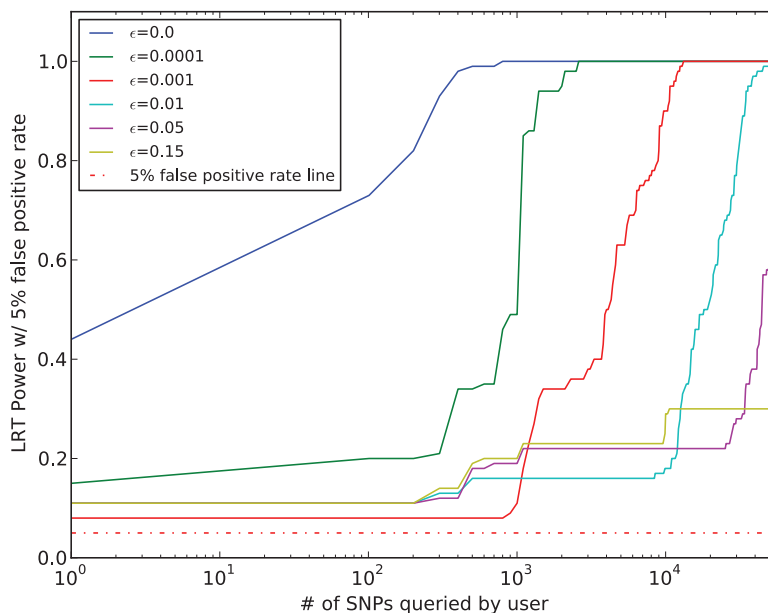
Figure 4. “Optimal” re-identification attack in beacon with S2 . Different power rates per number of SNPs queried (with rare-first logic) from a beacon with mitigation S2 by an adversary with knowledge on \epsilon and on AFs from the 1000 Genomes project. Different colors for different values of \epsilon .
