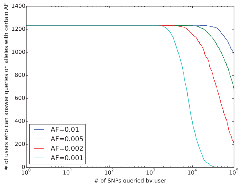
Figure 5. Budget evaluation in beacon with S3 . Behaviors of individual budgets per number of SNPs queried according to the typical user's query profile obtained from ExAC log data. The cyan curve represents the number of individuals with enough budget to answer "Yes" to queries targeting alleles with AF = 0.001. Red, green, and blue curves correspond to 0.002, 0.005, and 0.01, respectively.
