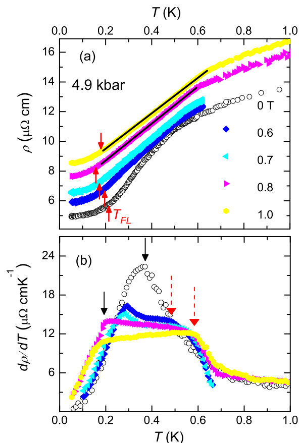
FIG. 9. (a) Temperature variation of the electrical resistivity at different magnetic fields for p = 4.9 kbars. For better readability, \rho(T) data are shifted by +0.5 at 0.6 T, +1 at 0.7 T, +2 at 0.8 T, and +3 at 1 T ( \mu\Omega \text{ cm} ). The straight line indicates the most extended linear temperature range ascribed to non-Fermi liquid behavior. The arrows indicate the Landau-Fermi liquid temperature T_{FL} (see text). (b) Temperature dependence of the first derivative of electrical resistivity d\rho/dT . Solid and dashed arrows indicates putative T_N and T_Q , respectively.
