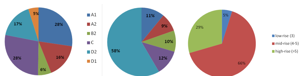
Figure 5. Distribution per structural typology for (left) Sion and (center) Martigny sample; (right) per height for both cities sample
