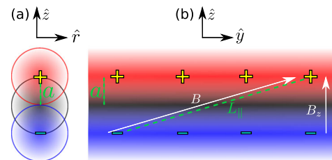
FIG. 4. Schematic of blob density profile (black) with the associated potential dipole (red and blue) on the poloidal cross section (a) and along the toroidal direction (b), with the parallel connection length L_{\parallel} and the blob size a indicated.
