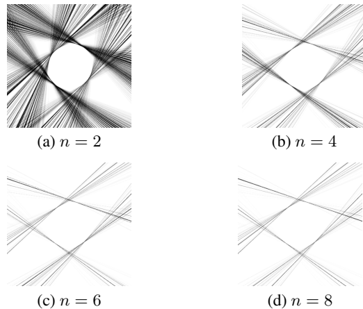
Fig. 6. Sampled distribution of the room geometry estimated with the Algorithm 2 at different steps. The lightness level of the lines presents the probability of the estimation: darker line—higher probability that the line corresponds to the wall.
