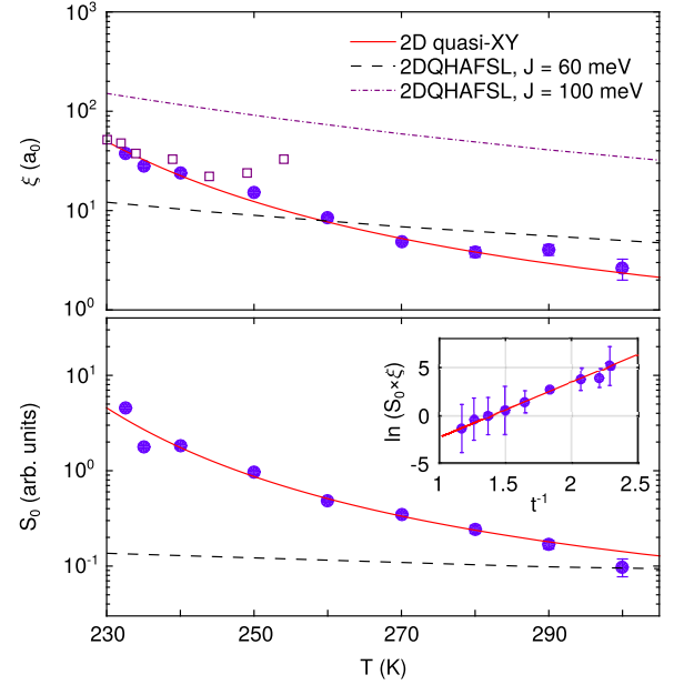
FIG. 3. (Color online) Temperature dependence of the correlation length (top panel) and the amplitude (bottom panel) of the critical scattering for Sr 2 IrO 4 as solid circles. Open squares are data taken from Fujiyama [21] divided by a_0 . QMC results with J = 60 meV (100 meV) as a dashed line (dotted-dashed line) Ref. [18]. Solid line: Fit of a 2D model with XY anisotropy, as discussed in text. Inset: Linear scaling of \ln(\xi S_0) \sim (3 - \eta)bt^{-1} .
