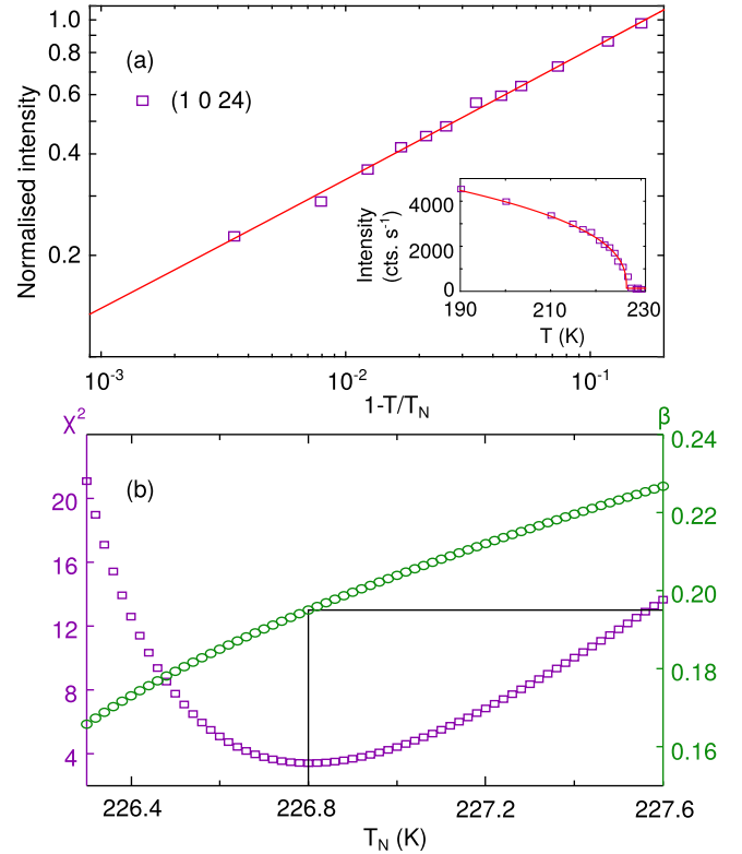
FIG. 1. (Color online) Order parameters of the magnetic critical scattering in \text{Sr}_2\text{IrO}_4 : (a) Integrated intensity and power-law fit (solid line) corresponding to best-fit values of T_N = 226.80(6) K and \beta = 0.195(4) . (b) Goodness of fit \chi^2 (purple squares) and the resulting exponent \beta (green circles) as a function of the chosen ordering temperature T_N . The fit in (a) corresponds to the minimum in \chi^2 .
