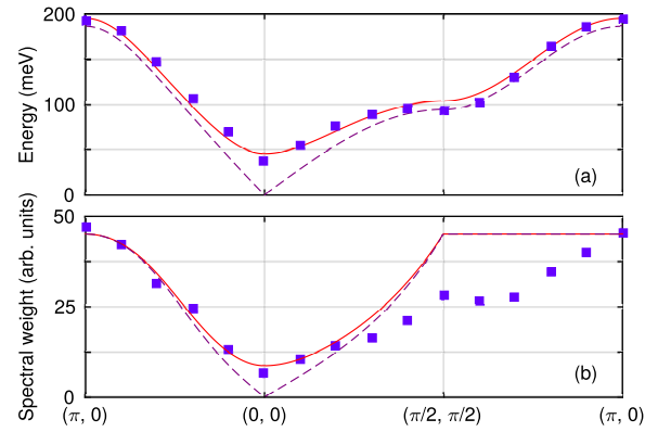
FIG. 4. (Color online) Fit of the anisotropic 2D Heisenberg model to the experimental single magnon dispersion. Squares: (a) Energy and (b) spectral weight of the single magnon peak obtained from fitting RIXS data provided in Ref. [5]. Error bars are smaller than the displayed symbols. Solid and dashed lines: Best fit of gapped and gapless modes to experimental data with \tilde{J} = 57(7) meV, J_2 = -18(3) meV, J_3 = 14(2) meV, and \Delta_\lambda = 0.08(1) .
