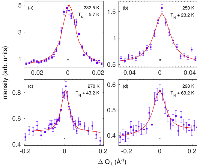
FIG. 2. (Color online) Critical scattering data for T > T_N obtained in scans performed perpendicular to the wave-vector transfer \mathbf{Q} of the appropriate antiferromagnetic Bragg peak. Solid lines: Fits of a Lorentzian line shape convoluted with the experimental resolution. The horizontal bars under the peaks represent the resolution full width at half maximum.
