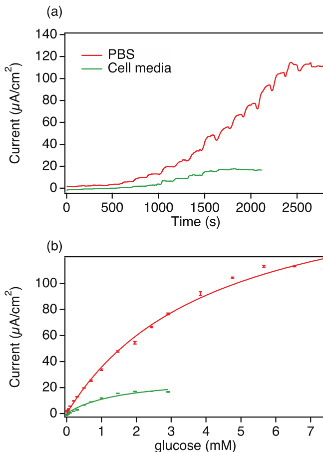
Fig. 3. (a), Chronoamperometry of the biosensor to different concentration of glucose in PBS (red) and in cell media (green); (b) Kinetics of the GOx immobilized on the electrodes in PBS (red) and in cell media (green); applied potential +0.30 V vs Ag|AgCl|Cl^- .
