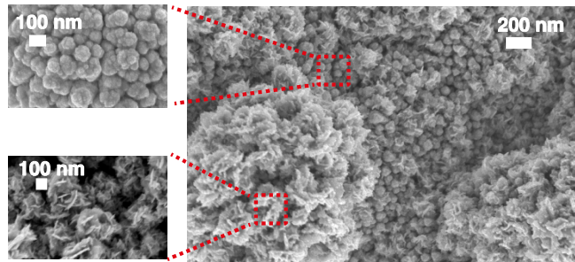
Fig.1. SEM image of Pt nanoflowers onto Pt nanospheres. Magnifications of Pt nanospheres (top left) and Pt nanoflowers (bottom left).
