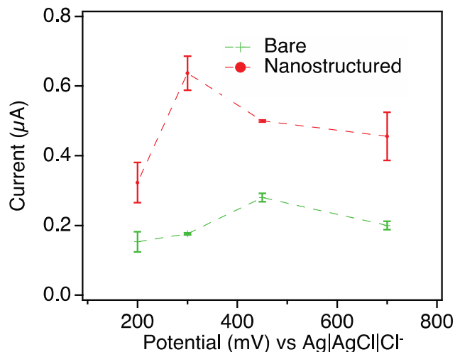
Fig. 2. Effect of applied potential on the amperometric response at bare (green) and at \text{Pt}_{\text{NS}}\text{Pt}_{\text{NF}} (red) electrode towards the detection of 20 \mu\text{M} \text{H}_2\text{O}_2 .
