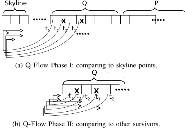
Fig. 2: The parallel phases of the Q-Flow algorithm: comparing to known skyline points (a), then other survivors (b).
