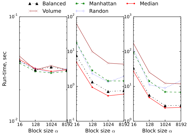
Fig. 9: Effect of pivot selection in Hybrid ( n = 1M , d = 12 )
