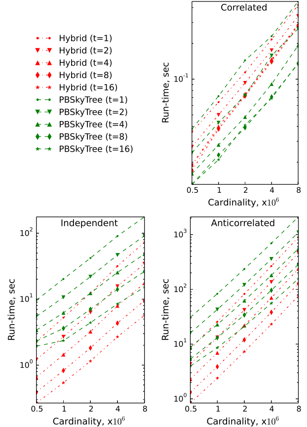
Fig. 13: Parallel Scalability in Hybrid w.r.t. n ( d = 12 ).
