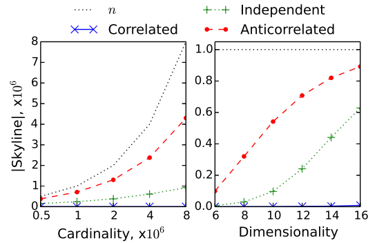
Fig. 4: Skyline sizes in synthetic data.
