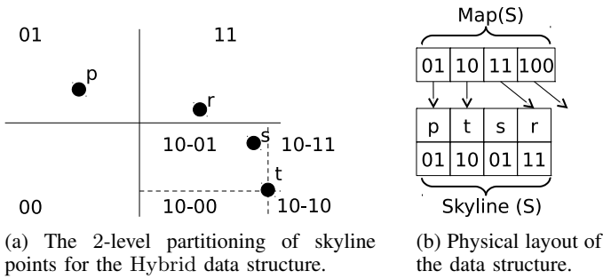
Fig. 3: Skyline points data structure in Hybrid.
