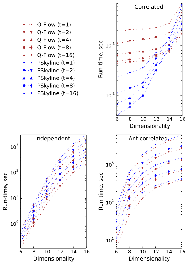
Fig. 10: Q-Flow versus PSkyline w.r.t. d ( n = 1M ).
