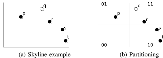
Fig. 1: (a): p, r, s, t are in the skyline, but not q : it has higher x - and y -values than p . (b): partitioning reveals incomparability and refines the probability of a point dominating another.
