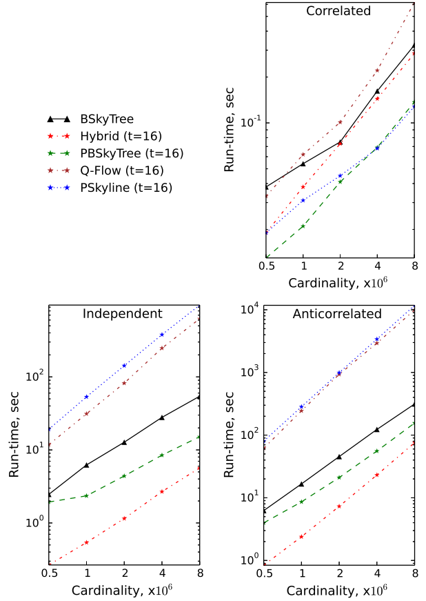
Fig. 6: State-of-the-art performance w.r.t. n ( d = 12 ).
