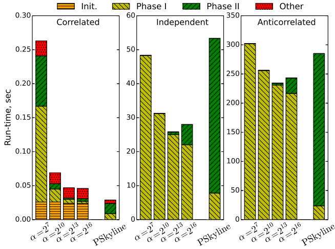
Fig. 7: Effect of \alpha in Q-Flow with varied \alpha ( n = 1\text{M} , d = 12 )
