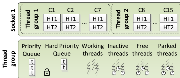
Figure 6: NUMA-aware task scheduler design.
