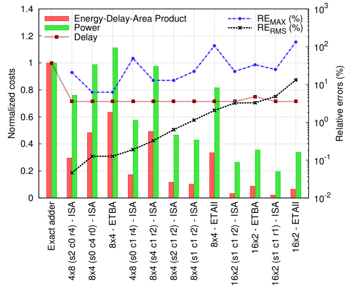
Fig. 7. Design costs and relative errors of selected ISA synthesized at 5 GHz. Delays are shown as the fastest exact adder cannot fit the 5 GHz constraint. 16x2 ETBA suffers from a drop of efficiency exactly at synthesized speed (q.v. section III-B), it is replaced with a slightly slower one for fair comparison.
