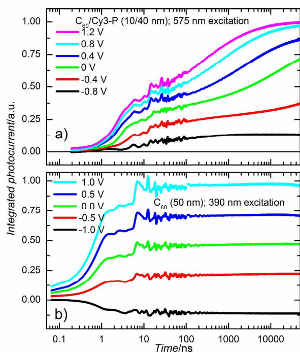
Figure S4. Integrated photocurrent versus time obtained by integral mode time of flight measurement; a) C 60 /Cy3-P (10/40), 575 nm excitation (0.2 μJ/cm 2 ); b) pristine C 60 film, 390 nm excitation (0.7 μJ/cm 2 ). Labels indicate different bias.
