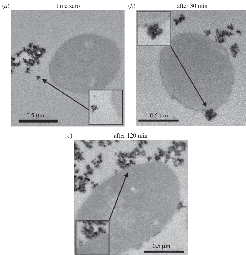
Figure 12. TEM of TiO 2 -PES 5% (hydrothermal) interacting with the E. coli cell wall in the dark at (a) time zero (b) time 30 min (c) time 120 min. For more details, see text.
