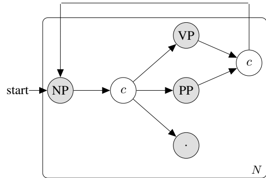
Figure 4. The constrained language model for generating a description given the predicted phrases for an image.
