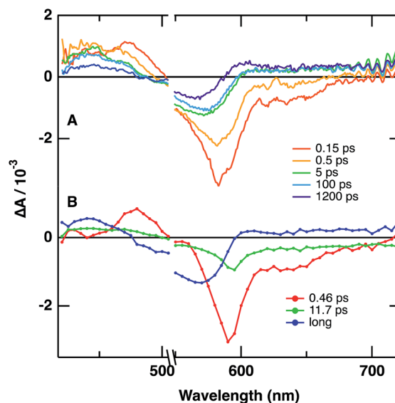
Fig. 3 (a) Transient absorption spectra at various time delays after 530 nm excitation for pristine Cy3-B and (b) amplitude spectra associated with the time constants resulting from the multiexponential global analysis for pristine Cy3-B.
