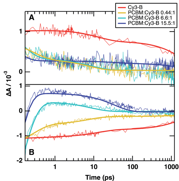
Fig. 5 Dynamics recorded after 530 nm excitation for pristine Cy3-B and various PCBM loadings for (a) 440 nm (Cy3 excited and reduced states) and (b) 550 nm (Cy3 GSB and oxidized state) probe wavelengths. The solid lines represent the result of the best multi-exponential fit.
