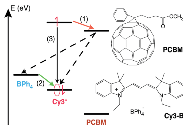
Fig. 1 Schematic layout of energy levels and electron transfer processes following Cy3 photoexcitation in pristine Cy3-B and blends with PCBM. (1) Electron transfer from Cy3 LUMO to PCBM; (2) reductive quenching of the Cy3* excited state by the tetraphenylborate counter-anion (e - transfer from BPh 4 to the Cy3 HOMO); (3) deactivation of Cy3* through radiative and non-radiative pathways. Back-electron transfer and charge recombination at tetraphenylborate|PCBM junctions appear as dotted lines. The molecular structures of the investigated materials are shown on the right.
