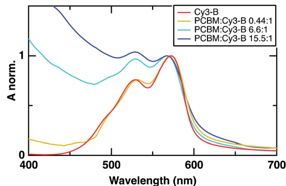
Fig. 2 Normalized steady-state absorption spectra of the pristine Cy3-B film and the various blends with PCBM.
