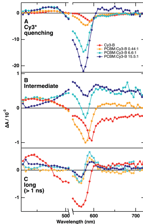
Fig. 6 Associated amplitude spectra resulting from the multi-exponential global analysis for various investigated samples. (a) is the excited state quenching, (b) is the intermediate time scale (order of 100 ps) and (c) is the long time scale (> 1 ns).
