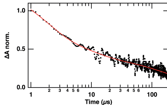
Fig. 4 Dynamics recorded at a 450 nm probe after 530 nm excitation for pristine Cy3-B. The solid line is the best fit of experimental data points.
