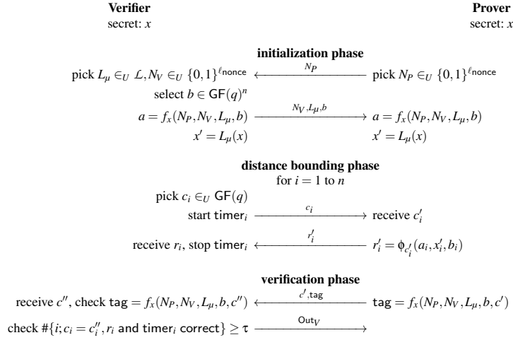
Fig. 1. The DBopt Distance-Bounding Protocols
