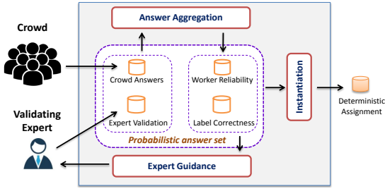
Figure 3: Framework for guided answer validation
