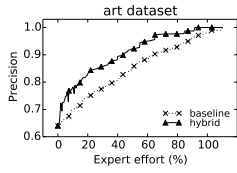
Figure 11: Guiding with expert mistakes
