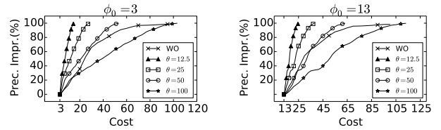
Figure 12: Collect more crowd answers vs. validate more
