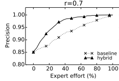
Figure 19: Effect of worker reliability
