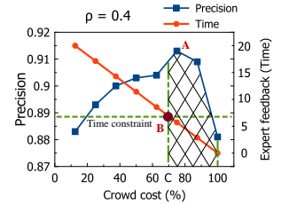
Figure 14: Balance with time and budget constraints
