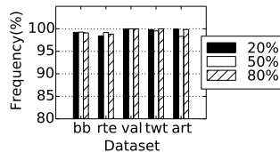
Figure 7: i -EM on guiding
