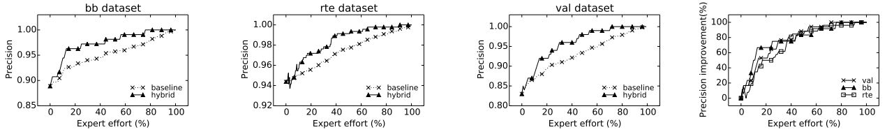
Figure 10: Effectiveness of guiding
