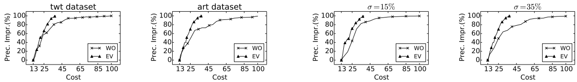
Figure 21: Effect of question difficulty on cost
