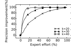
Figure 17: Effect of number of labels
