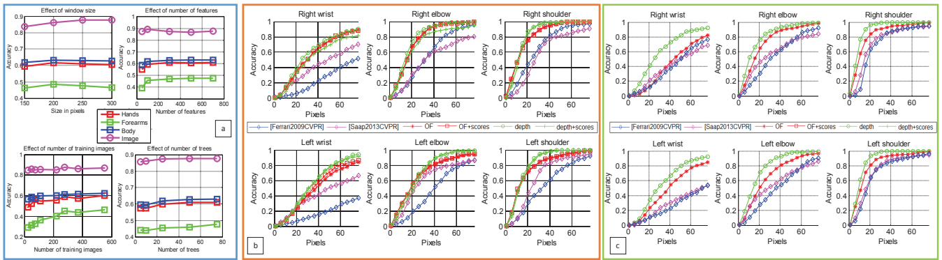
Figure 5: Parameter sensitivity of the classifier. b: Accuracy of the regressor in our job database, compared against [9] (blue) and [22] (magenta). c: Results in ChaLearn2011, compared against [9] (blue) and [22] (magenta). Best viewed in PDF in high zoom.
