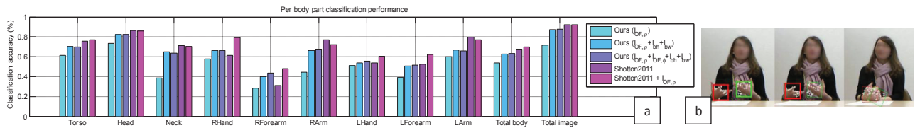
Figure 4: Left: Results of our method versus [25] , when trained with the same number of images: Reported as classification rates for every body segment. Performance is asymmetrical as the camera is slightly off-center. Right: Integration with the KLT tracker example . Reliable detections are represented with a thick box. The good features to track are shown as white crosses.
