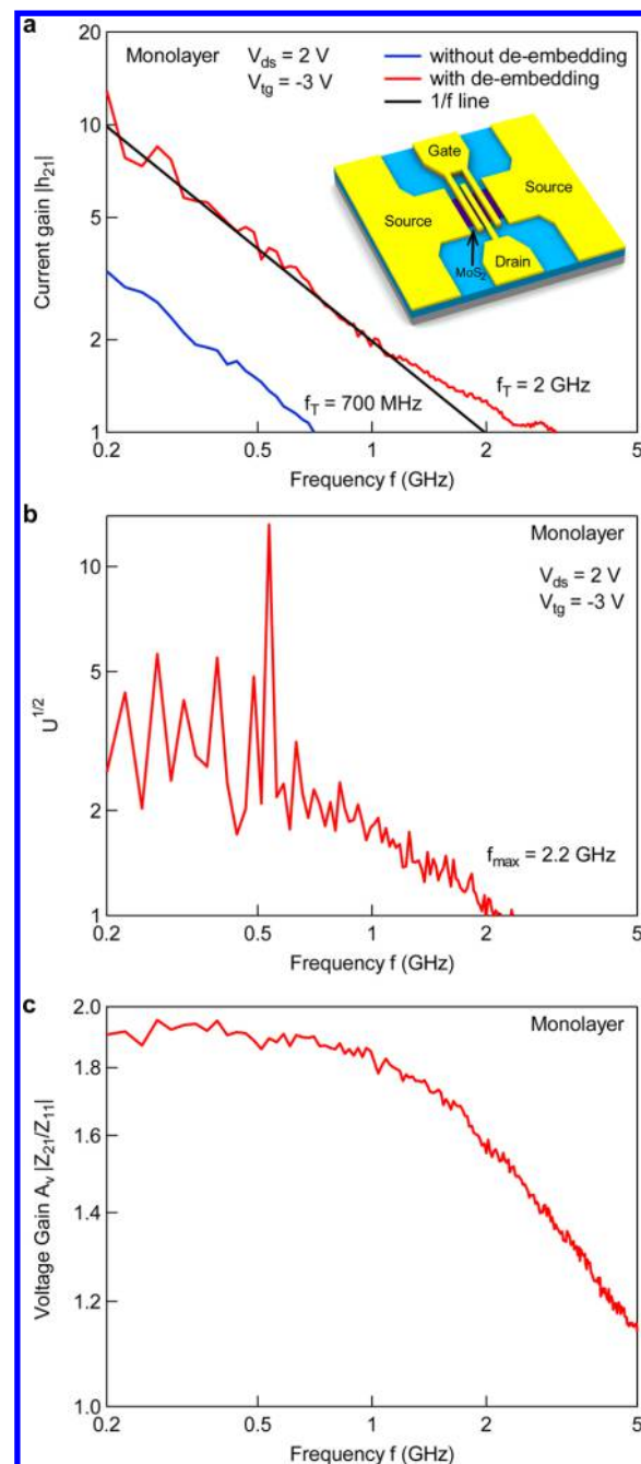
Figure 4. RF performance of MoS 2 transistors. (a) Small-signal current gain h_{21} as a function of frequency for devices based on single-layer MoS 2 with the cutoff frequency f_T = 2 GHz. (b) Mason's unilateral gain U as a function of frequency. Maximum frequency of oscillation f_{\text{max}} = 2.2 GHz is extracted. (c) Voltage gain |Z_{21}/Z_{11}| as a function of frequency showing gain higher than 1 up to 5 GHz. Adapted with permission from ref 16. Copyright 2014 American Chemical Society.
