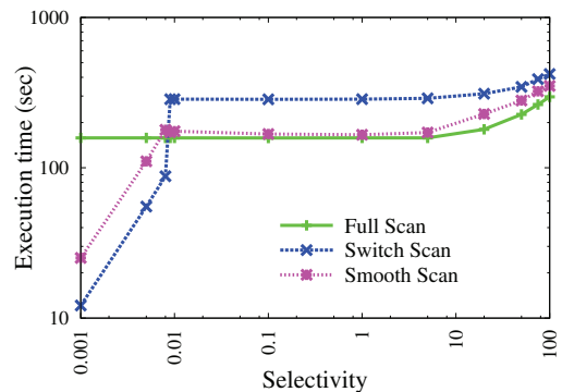
Fig. 11: Switch Scan Performance Cliff and Overall Benefit.
