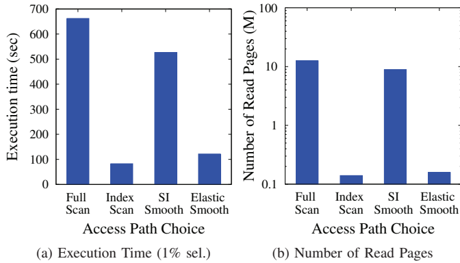
Fig. 8: Handling Skew.
