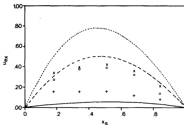
FIG. 1. Excess energy of mixing. The curves are the results of perturbation theory. —: \mu^2 = 1 ; - - : \mu^2 = 3 and ···: The simulation results are marked as points. \mu^2 = 4 , + : \mu^2 = 1 ; \square : \mu^2 = 3 and \times : \mu^2 = 4 .
