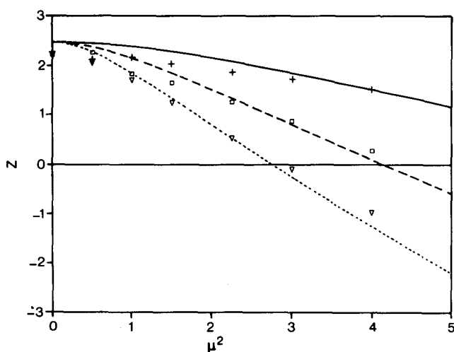
FIG. 6. Compressibility factor Z = \beta P / \rho . The points give the results of simulation; the curves the predictions of perturbation theory. —: x_s = 0.333 ; - - : x_s = 0.667 and ···: x_s = 1.000 , + : x_s = 0.333 ; □: x_s = 0.667 and ▽: x_s = 1.000 .
