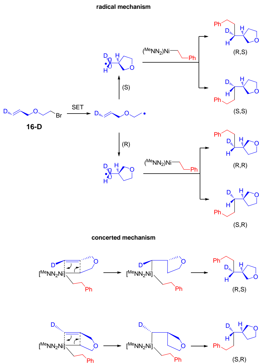
Scheme 3. Stereochemical outcomes of radical or concerted mechanism.
