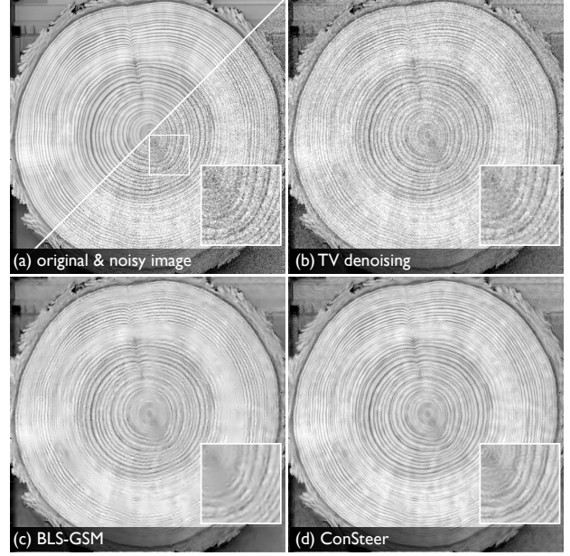
Fig. 1: Comparison of denoising results for wood: (a) original and noisy image (SNR=15 dB); (b) TV denoising (SNR=19.12 dB); (c) BLS-GSM denoising (SNR=22.46 dB); (d) ConSteer denoising (SNR=23.05 dB).
