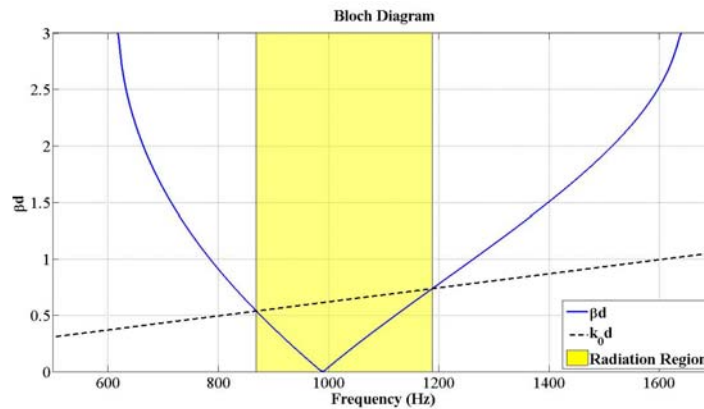
Figure 3. Dispersion diagram
