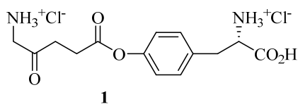
Figure 1. Structure of 5-ALA-Tyr ester ( 1 ).
