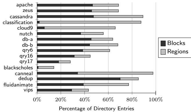
Figure 12: Breakdown of the average number of block and region entries within the DGD 8way directory.
