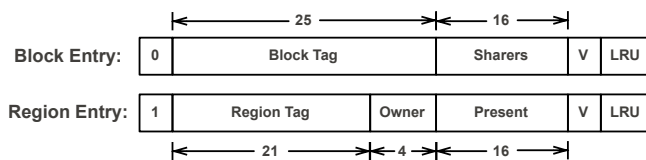
Figure 5: Formats of block and region entries in DGD.
