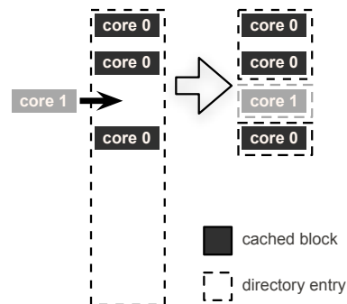
Figure 1: Example of splitting an iMGD directory entry.
