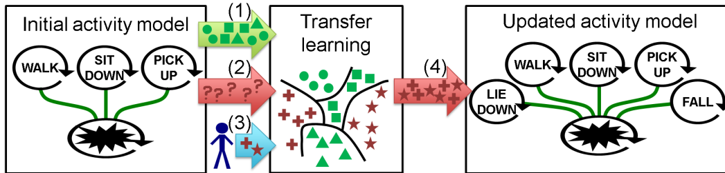
Figure 1. Schematic overview of our approach to combine activity tracking with transfer learning. In surveillance videos, an initial model recognizes familiar activities (1) or detects abnormalities (2). Together with minimal human interaction (3), the transfer learning algorithm returns labels (4) such that the activity model can be extended with new classes.
