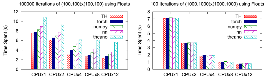
Fig. 4. Benchmarks of matrix multiplication performance using C, Torch7 torch package, nn package in Torch7 , Numpy and Theano . Tests were conducted on a machine with two Intel Xeon X5690 CPUs with 6 computational cores in each CPU. Hyper-threading was disabled. We considered multi-thread computation using 1, 2, 4, 8 and 12 CPU cores. Performance is given in seconds of time spent for processing, therefore smaller is better.
