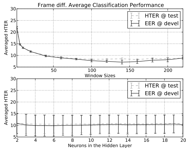
Fig. 5: Average performances for the dual optimization of RS3.
