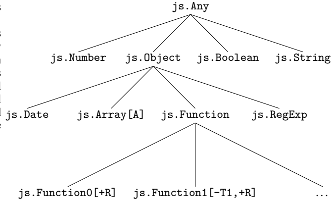
Figure 1. Core JS types in Scala.js
