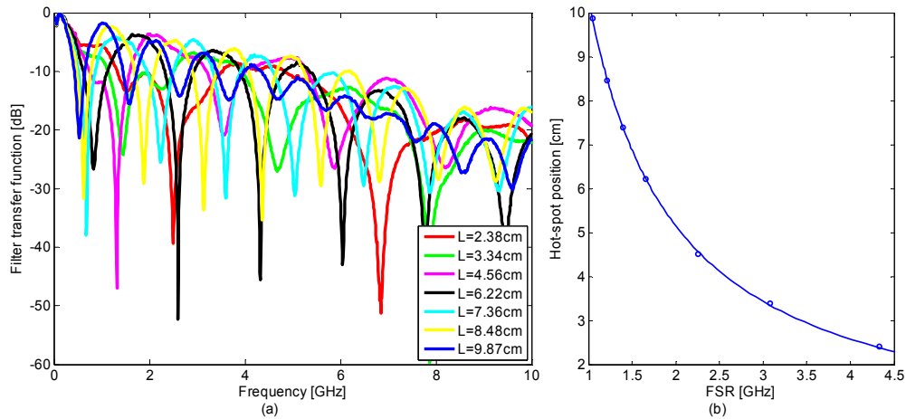
Fig. 3. a) Frequency response of the two tap filters achieved by placing a hot-spot on the FBG. Inset: Hot-spot position. Fig. 3. b) Comparison between the hot-spot position calculated from the IFT (dots) and the theoretical inverse linear relation (solid line).
