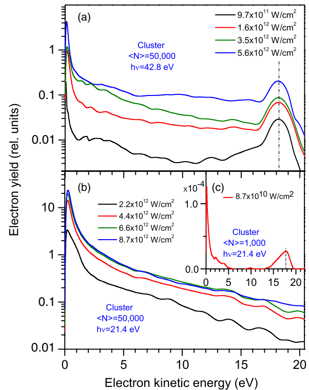
FIG. 2 (color online). Comparison of the photoelectron spectra of nanodroplets ( N \approx 50\,000 ) irradiated at 42.8 (a) and at 21.4 eV (b) photon energy for different power densities. The inset (c) depicts photoelectron spectrum of small nanodroplets ( N \approx 1000 ) at 21.4 eV for low power density.
