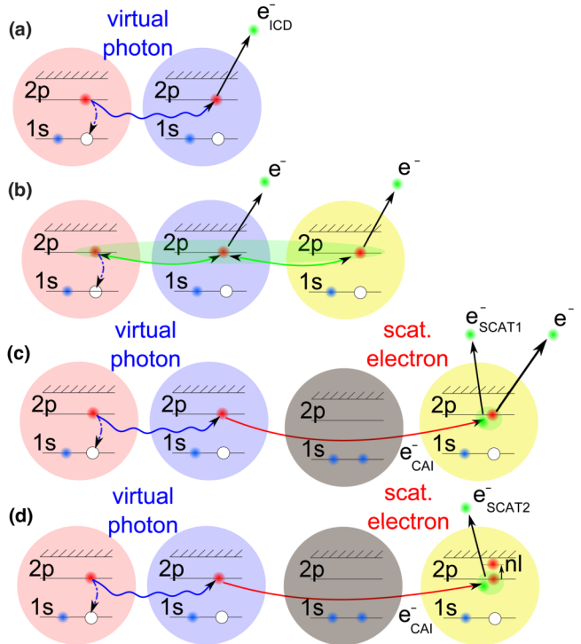
FIG. 1 (color online). Schematic diagrams of (a) ICD [9], (b) CAI type process involving three excited atoms, and (c),(d) CAI with electron scattering on a third neighboring excited atom (for details see text).
