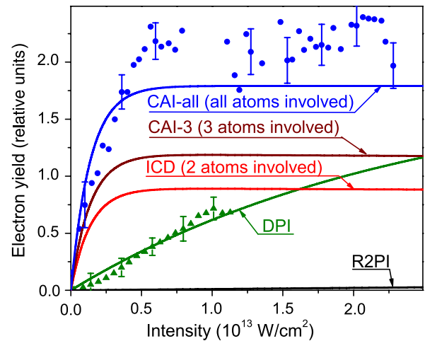
FIG. 3 (color online). Total electron yield vs FEL intensity for two different photon energies. Dots and triangles represent the experimental data at 21.4 and 42.8 eV, respectively. R2PI and ICD indicate theoretical electron yields for the resonant two-photon ionization process and ICD process at 21.4 eV, respectively. CAI-3 and CAI-all represent the theoretical yield for the CAI process where three and all excited atoms are involved, respectively. DPI shows the rate for the direct photoionization process at 42.8 eV ( \sigma_i \approx 2.89 Mb [31]). The theoretical electron yields are normalized to the experimental data through the DPI process.
