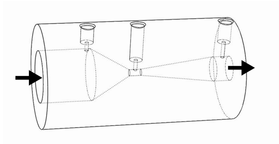
Fig. 2. 3D view of the Venturi tube
