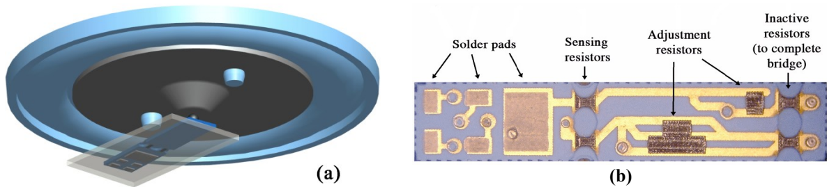
Fig. 3. (a) Elastomer membrane with reinforcing central structure mounted on LTCC cantilever sensor; (b) LTCC cantilever - bottom side.
