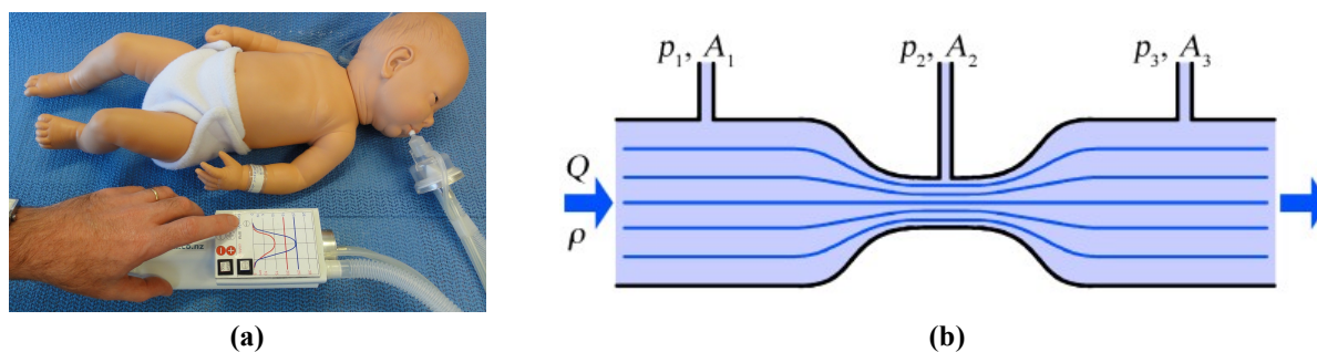
Fig.1. (a) neonatal respiratory assistance (source: www.kmedical.co.nz ); (b) 3D view & working principle of Venturi tube
