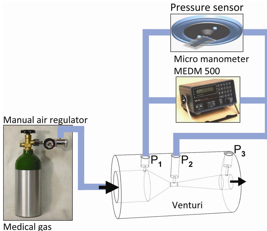
Fig 5. Experimental setup.
