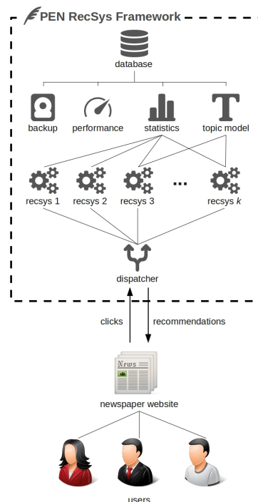
Figure 1: System architecture and components
