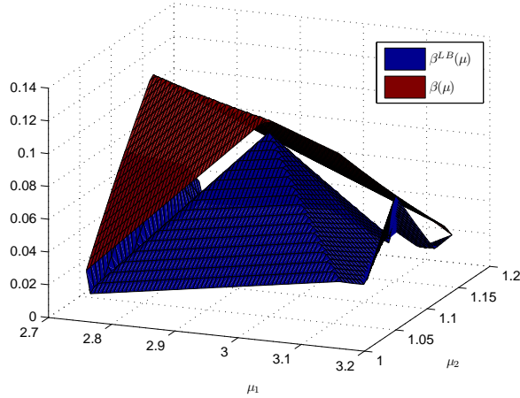
Figure 18: Electromagnetic Cavity problem ( \delta = 0.2 ): \beta(\mu) and \beta^{\text{LB}}(\mu) .
