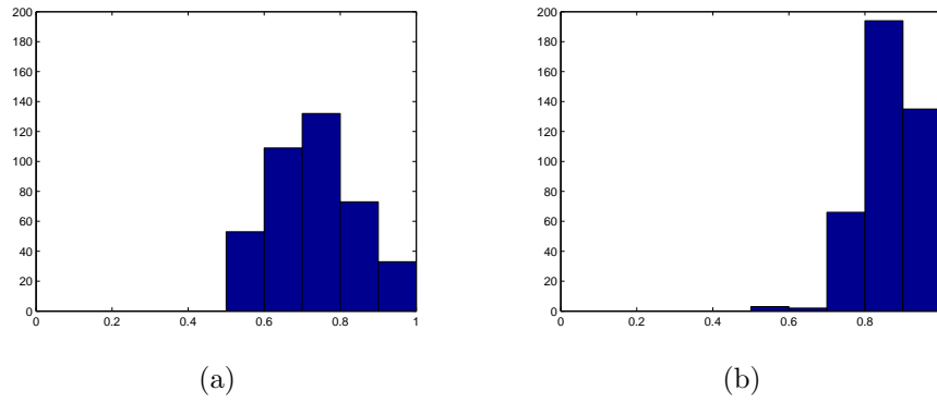
Figure 21: Convection–diffusion problem: Histogram for \Xi_{\text{test}} of (a) \beta^{\text{LB}}(\mu)/\beta(\mu) with \delta = 0.4 ; \min_{\mu \in \Xi_{\text{test}}} \frac{\beta^{\text{LB}}(\mu)}{\beta(\mu)} = 0.506 , \text{avg}_{\mu \in \Xi_{\text{test}}} \frac{\beta^{\text{LB}}(\mu)}{\beta(\mu)} = 0.7307 , and (b) \beta^{\text{LB}}_{\text{SCM}^2}(\mu)/\beta(\mu) ; \min_{\mu \in \Xi_{\text{test}}} \frac{\beta^{\text{LB}}_{\text{SCM}^2}(\mu)}{\beta(\mu)} = 0.572 , \text{avg}_{\mu \in \Xi_{\text{test}}} \frac{\beta^{\text{LB}}_{\text{SCM}^2}(\mu)}{\beta(\mu)} = 0.865 .
