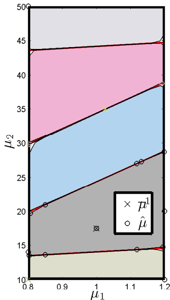
Figure 2: Anisotropic Wavespeed problem (greedy): Subdomains and the set C_{\bar{\mu}^1} .
