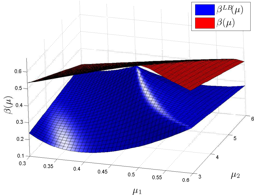
Figure 6: Microphone problem: \beta(\mu) and \beta^{\text{LB}}(\mu) .
