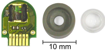
Fig. 5. Disassembled custom 0.8g optic-flow sensor, comprising a bare ADNS-9500 chip which is bonded to a custom printed circuit board (left). A lens holder (middle) is glued on top of the PCB and hosts a CAX100 lens with 10mm focal length (right).
