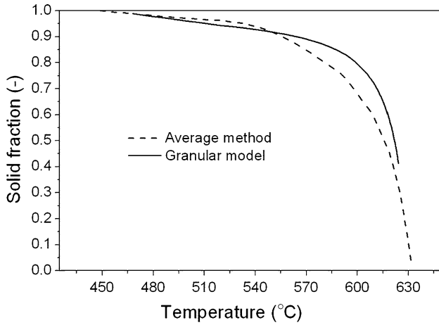
Fig. 4. Evolution of solid fraction with temperature as calculated with the granular model and reported in Ref. 10.
