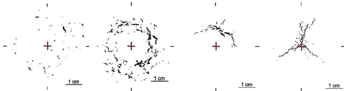
Fig. 2. Evolution of the hot tear morphology in a DC cast Al billet due to the increase in v_T from 90 mm/min to 120 mm/min. The center of the billet is indicated by the cross. 10
