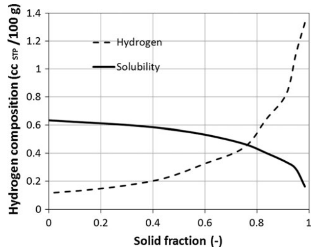
Fig. 1. Evolution of the hydrogen content in the liquid as a function of the fraction of solid, along with the equilibrium hydrogen saturation content for an AA5182 aluminum alloy. The initial composition was 0.1 \text{ cc}_{stp}/100 \text{ g} .
