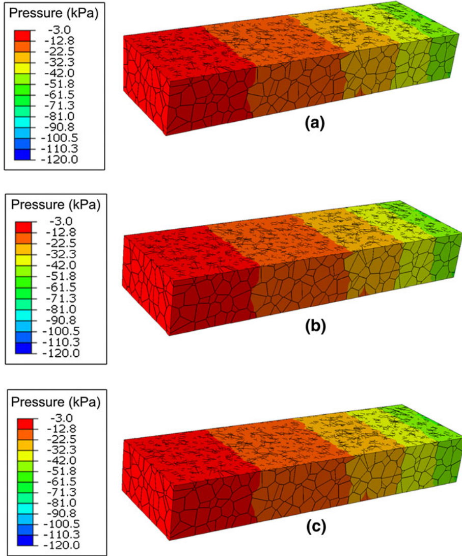
Fig. 7. Contour plots of the liquid pressure for v_T = 90 mm/min and \dot{\epsilon} = 0.0002 s ^{-1} at (a) \epsilon = 0.00053 ( t = 2.667 s), (b) \epsilon = 0.00106 ( t = 5.33 s), and (c) \epsilon = 0.00212 ( t = 10.66 s).
