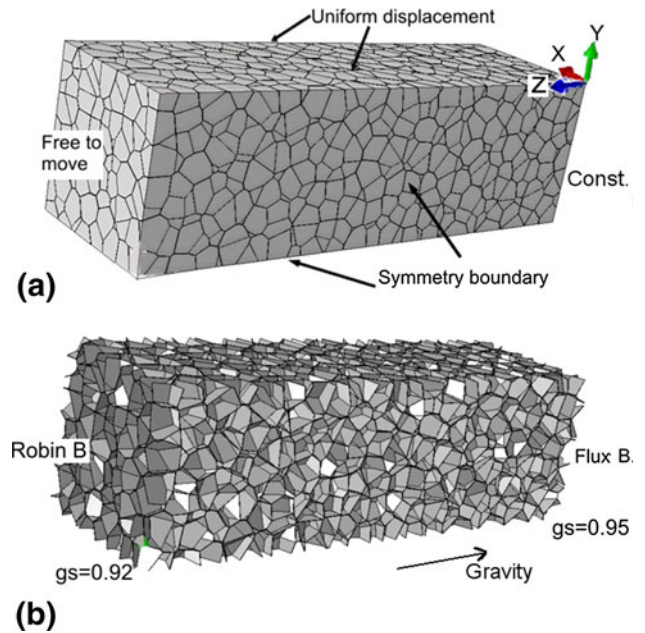
Fig. 5. Boundary conditions applied to the semisolid RVE containing 2430 grains for (a) SDM calculation and (b) FFM calculation. The solid elements are transparent in (b) to see the liquid film network in between the polyhedral grains.
