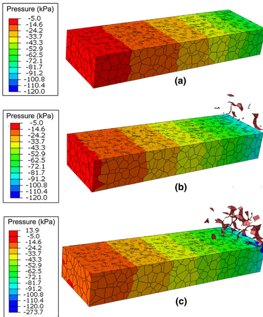
Fig. 6. Contour plots of the liquid pressure for v_T = 120 mm/min and \dot{\epsilon} = 0.0002 s -1 at (a) \epsilon = 0.00053 ( t = 2.667 s), (b) \epsilon = 0.00106 ( t = 5.33 s), and (c) \epsilon = 0.00212 ( t = 10.66 s).
