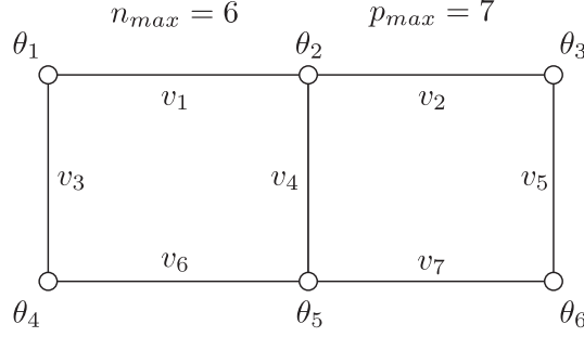
Figure 1: Simple network illustrating the leak flows and and water velocities in pipes. The total number of nodes is n_{max} = 6 and the total number of pipes is p_{max} = 7 .
