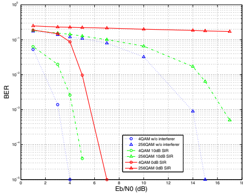
Fig. 8: BER for the D2D link under different level of interference
