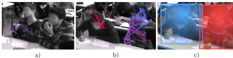
Fig. 1. Motion grouping. a) Individual motion vectors shown as purple arrows b) Grouped motion into motion tracks c) Marked student areas and centres of Gaussian probabilities of each student
